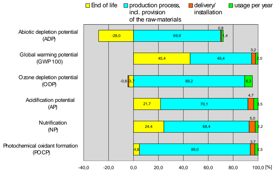
Graph 8: Relative contributions of the life cycle stages to the environmental impacts
