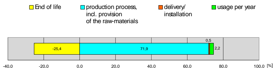
Graph 4: Relative contributions of the life cycle stages to the regenerative and non-regenerative primary energy consumption
